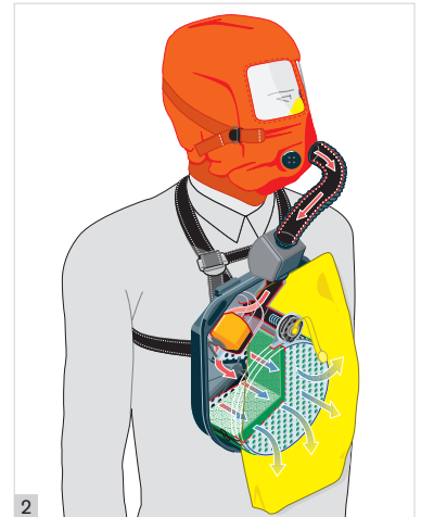
2 First exhalation cycle into breathing bag / Erste Ausatmung in den Atembeutel
